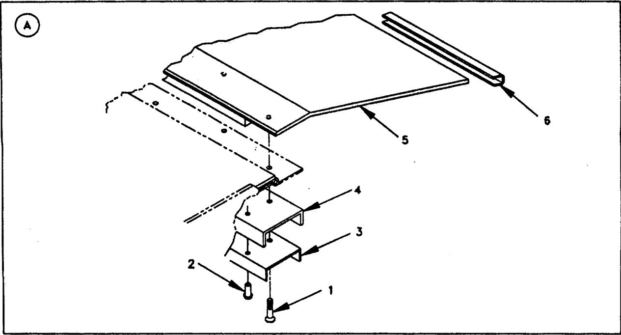
FIGURE 3 . RAMP ASSEMBLY (ISO TO TEMPER)
